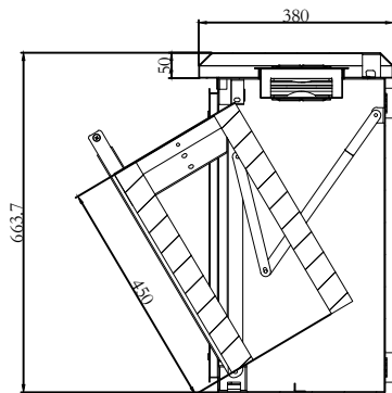
SECTION G-G
