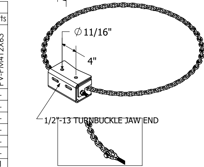
SINGLE SECTOR CHAIN MOUNT PV-CM1 SHOWN
