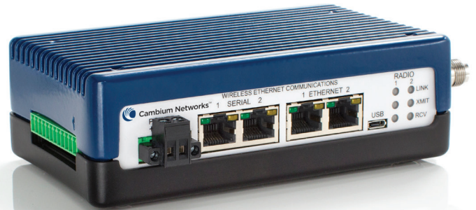
cnReach N500 700 MHz Radio
