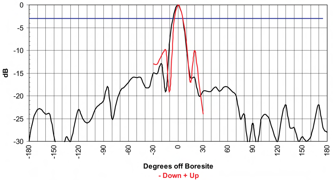
5.7 GHz Stinger Lite Pattern Azimuth - Elevation
