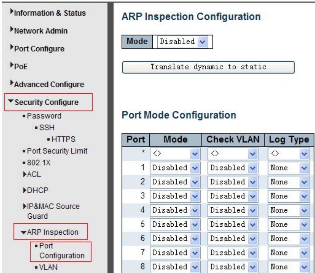
Figure 7-6 ARP Inspection Port Configuration Screen
