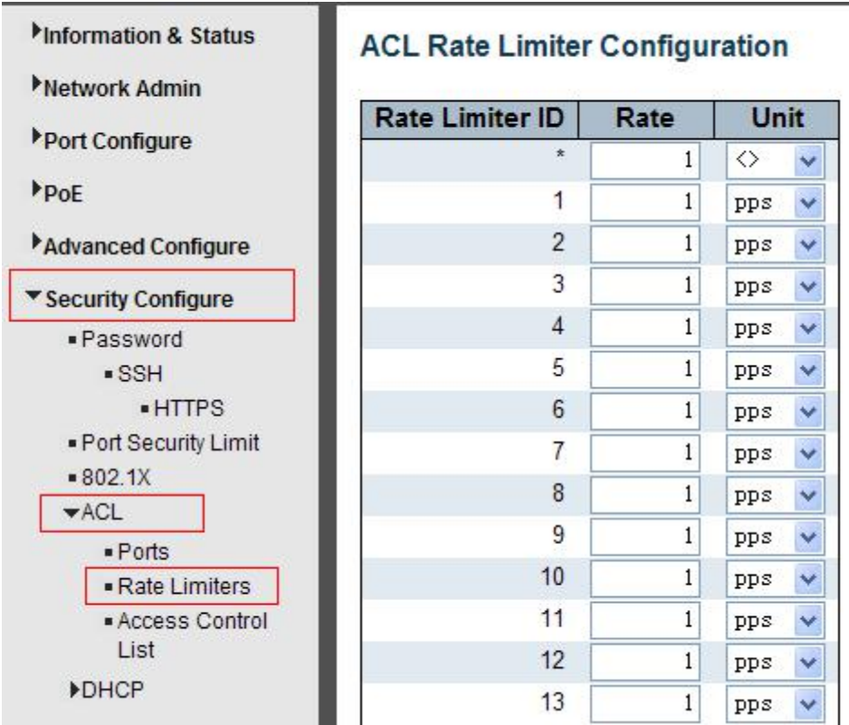
Figure 7-11 ACL Rate Limiters Configuration Screen
