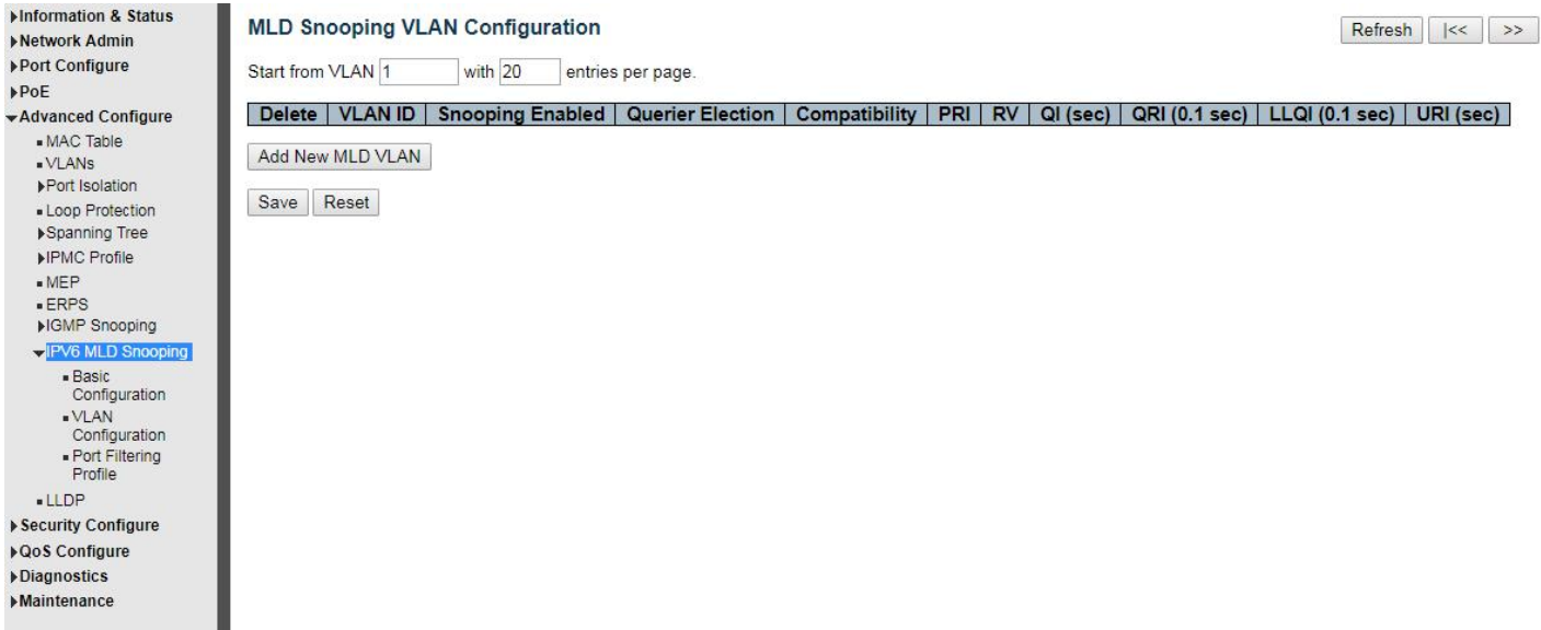
Figure 5-7-2 IPV6 MLD Snooping Setting
