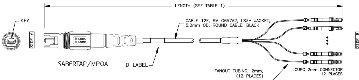
SABERTAP CONNECTOR ASSEMBLY
