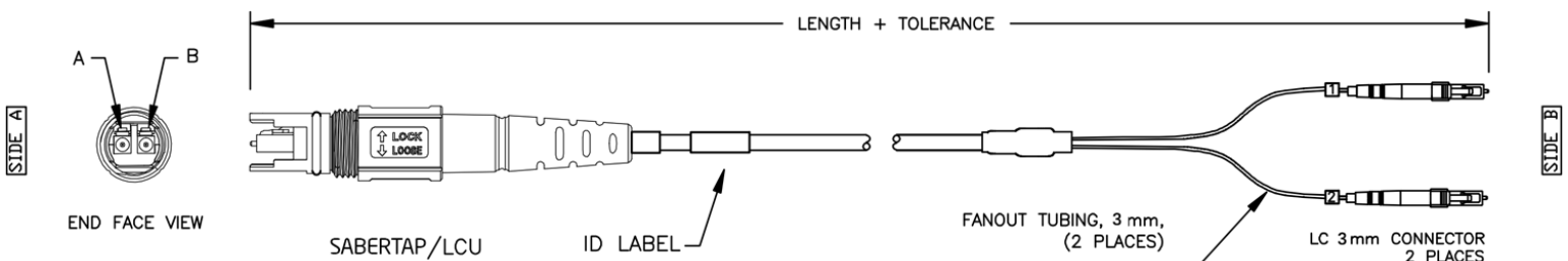
SABERTAP CONNECTOR ASSEMBLY
