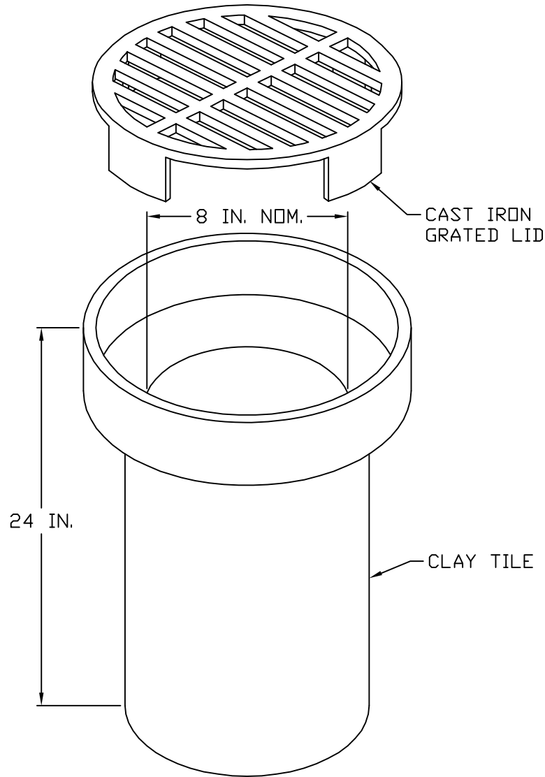
TILE WELL WITH GRATED COVER
