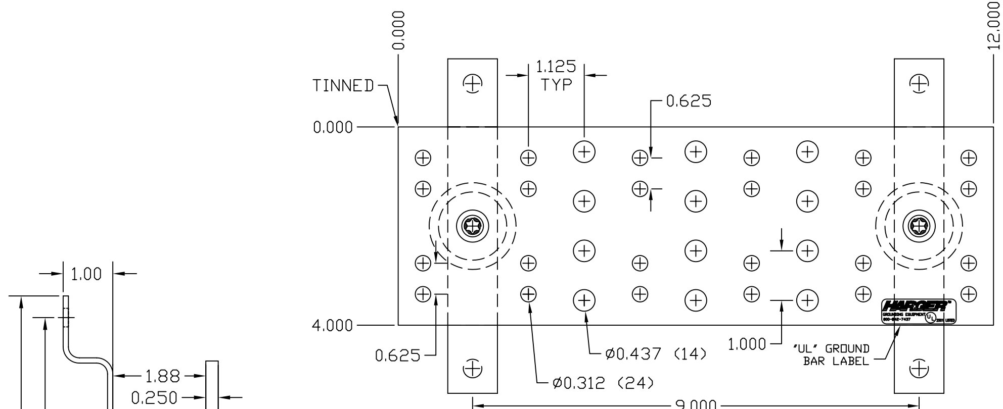
TINNED BICSI GROUND BAR ASSEMBLY
