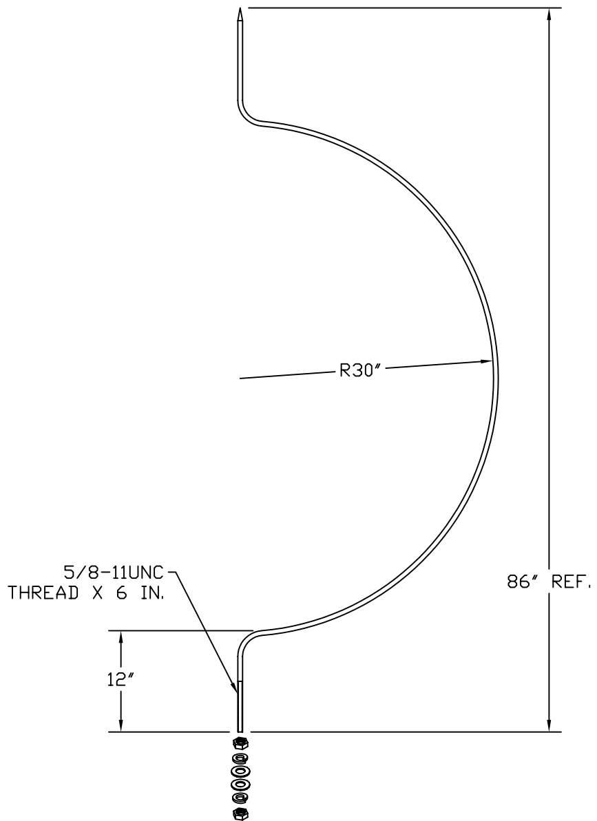
BENT COPPER CLAD AIR TERMINAL
