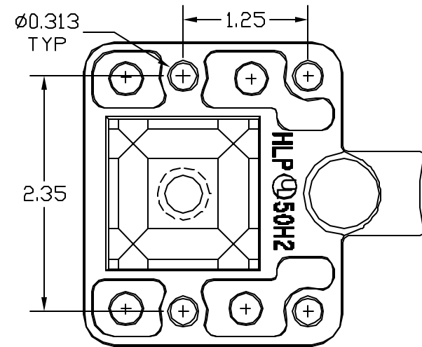
BASE DETAIL
