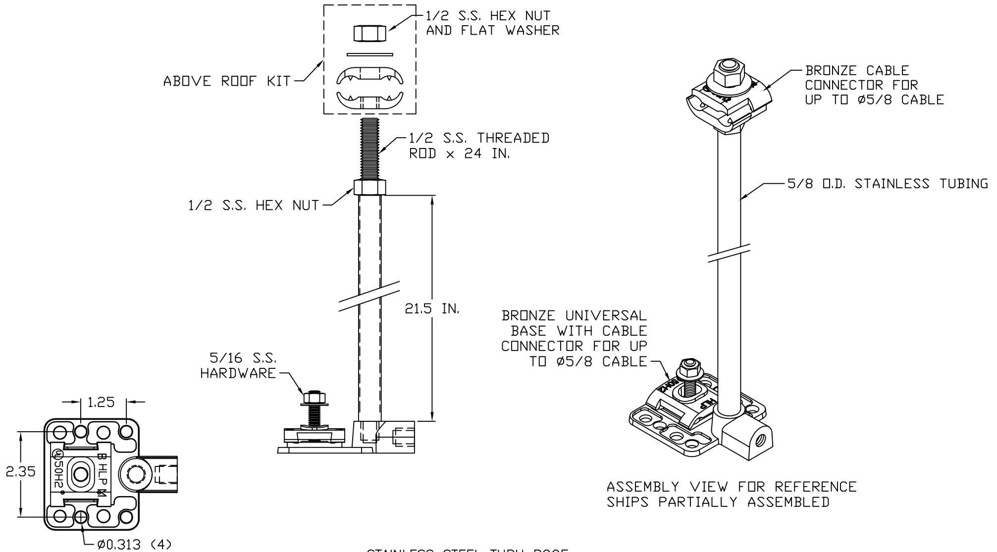
STAINLESS STEEL THRU ROOF COPPER TO COPPER
