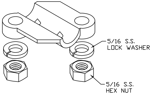
ASSEMBLY VIEW
