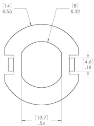
TABBED WASHER
